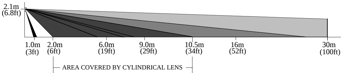
SIDE VIEW:*
