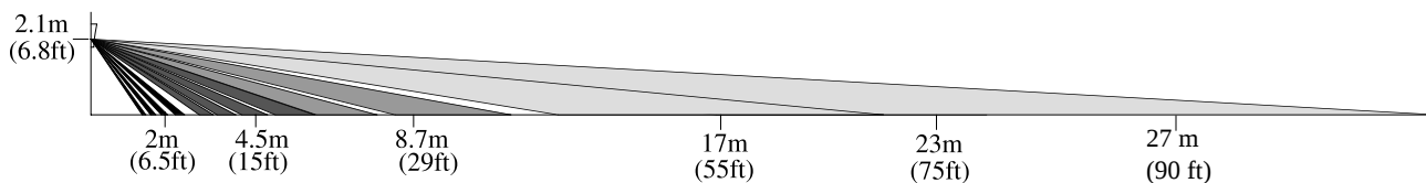
SIDE VIEW:*
